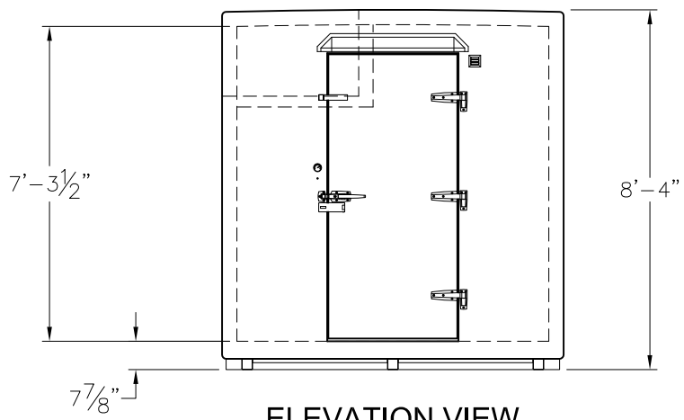
ELEVATION VIEW
