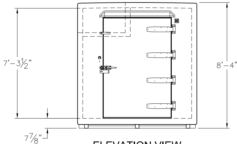
ELEVATION VIEW
