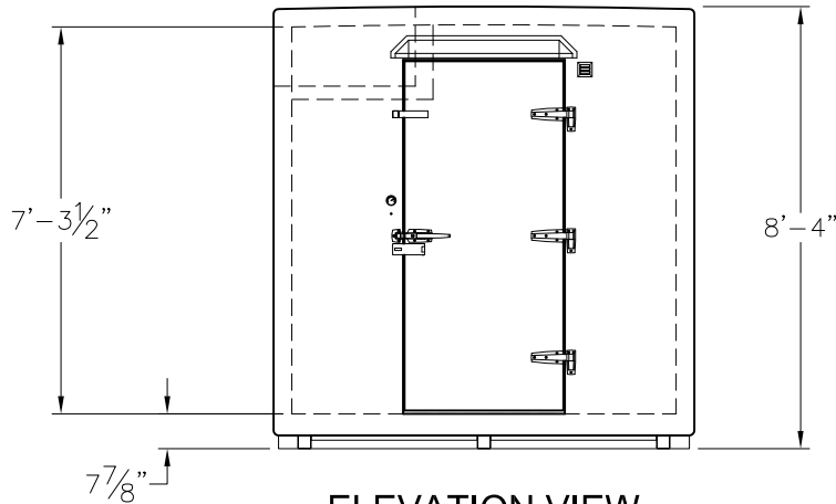
ELEVATION VIEW
