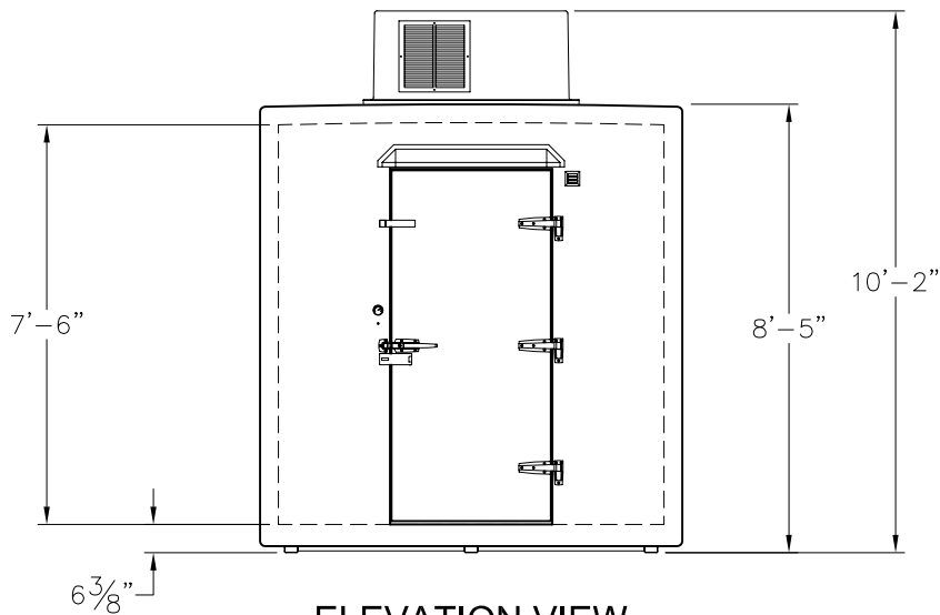
ELEVATION VIEW
